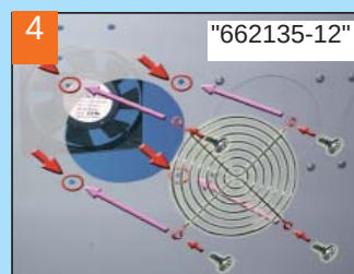
To screw a fan, a fan guard and roof panel by 4 points
